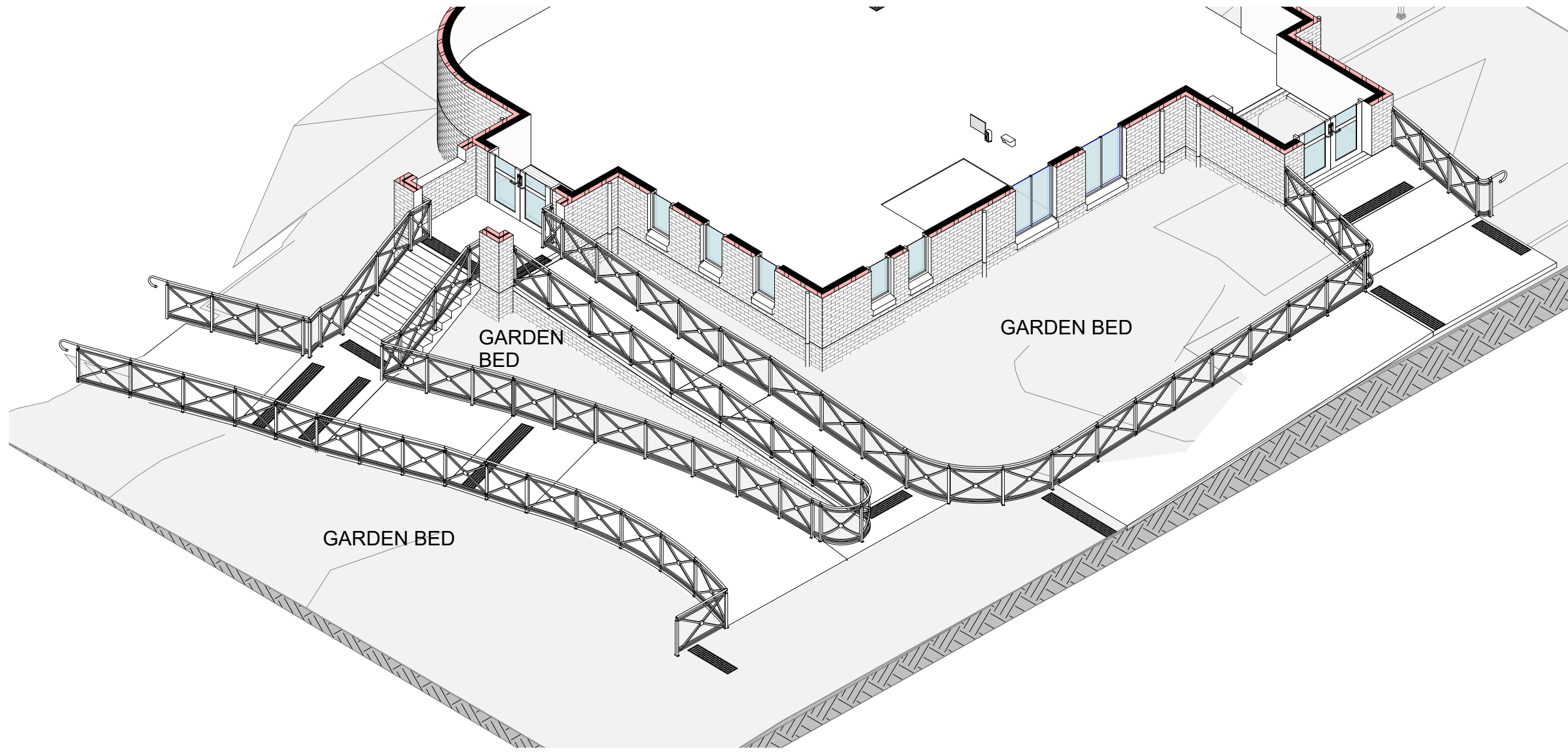
2 RAMP 1 ISOMETRIC VIEW PART 1
